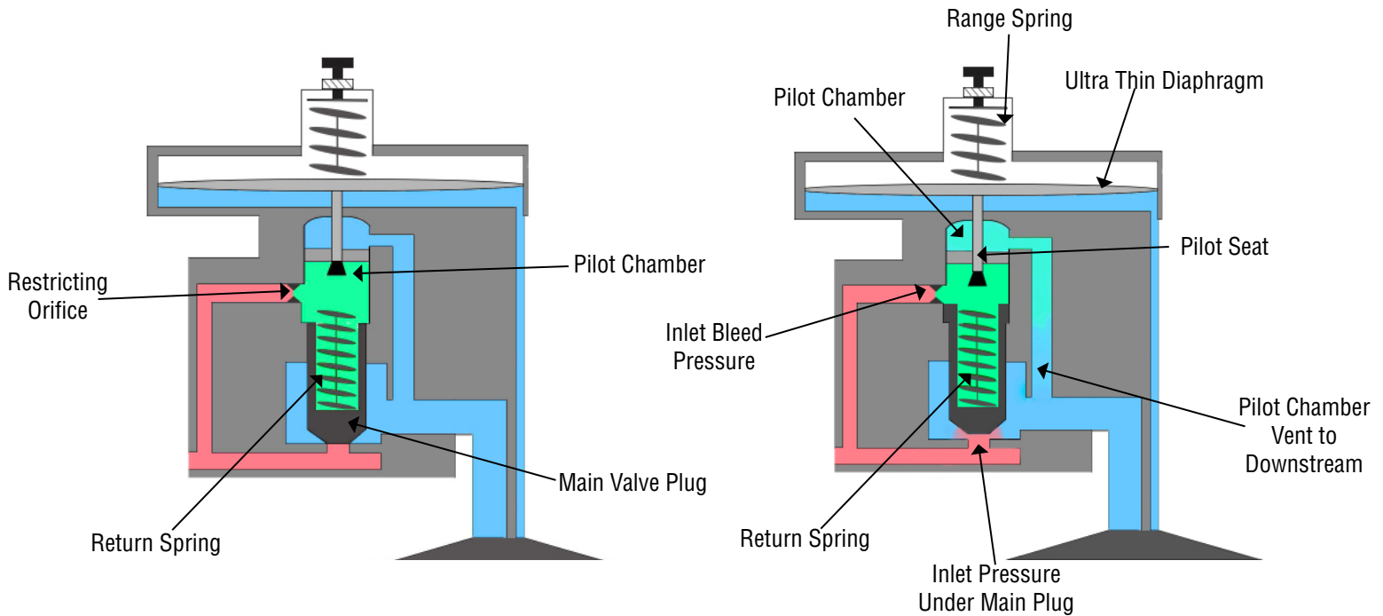
Figure 2 - Valve Open
